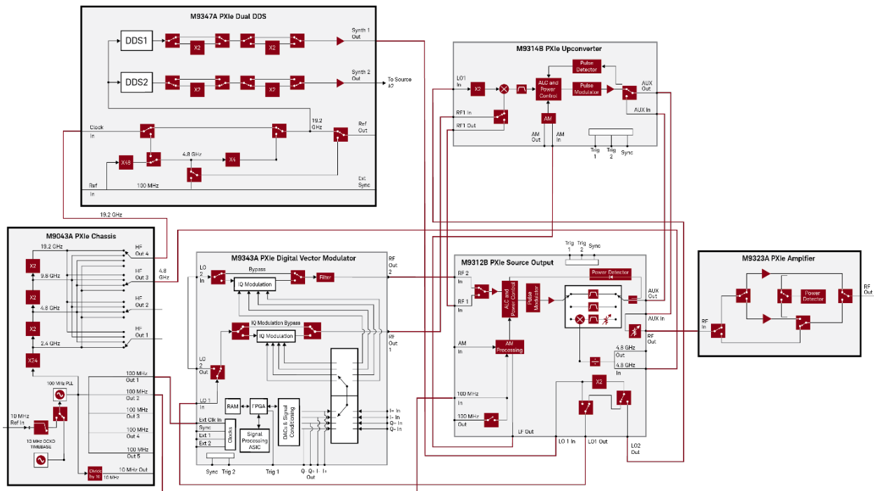
Figure 1. Block diagram for the VXG, a 44 GHz signal generator with 2 GHz RF bandwidth.
