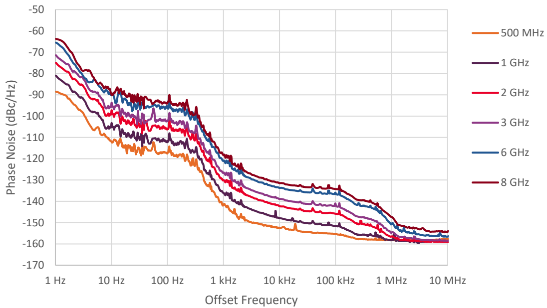
Measured SSB Phase Noise (Option EP4)
