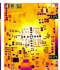
PCBA detection
