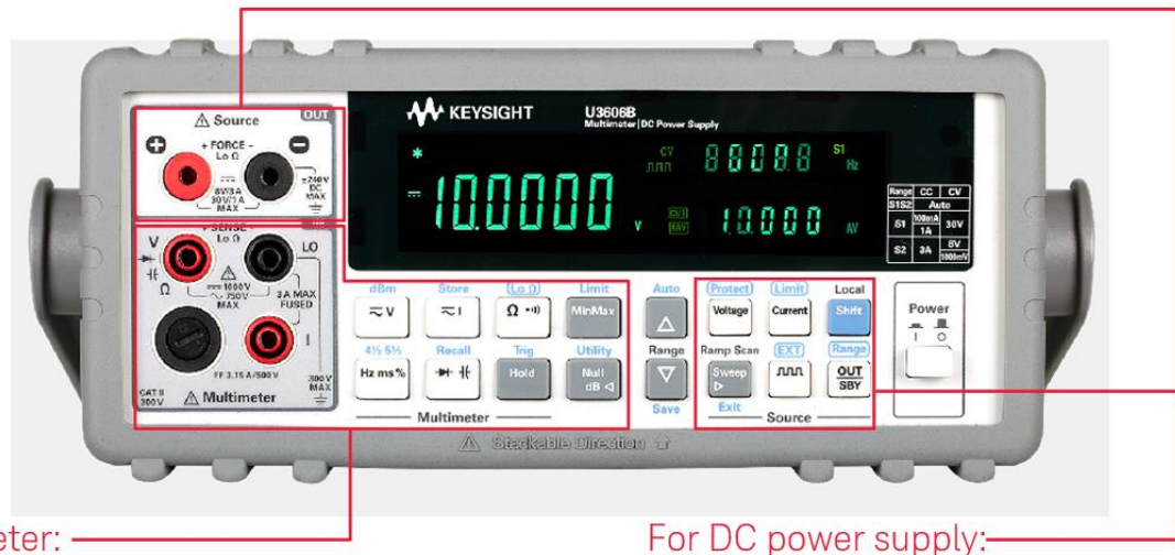
Figure 3. Front panel of the U3606B.
