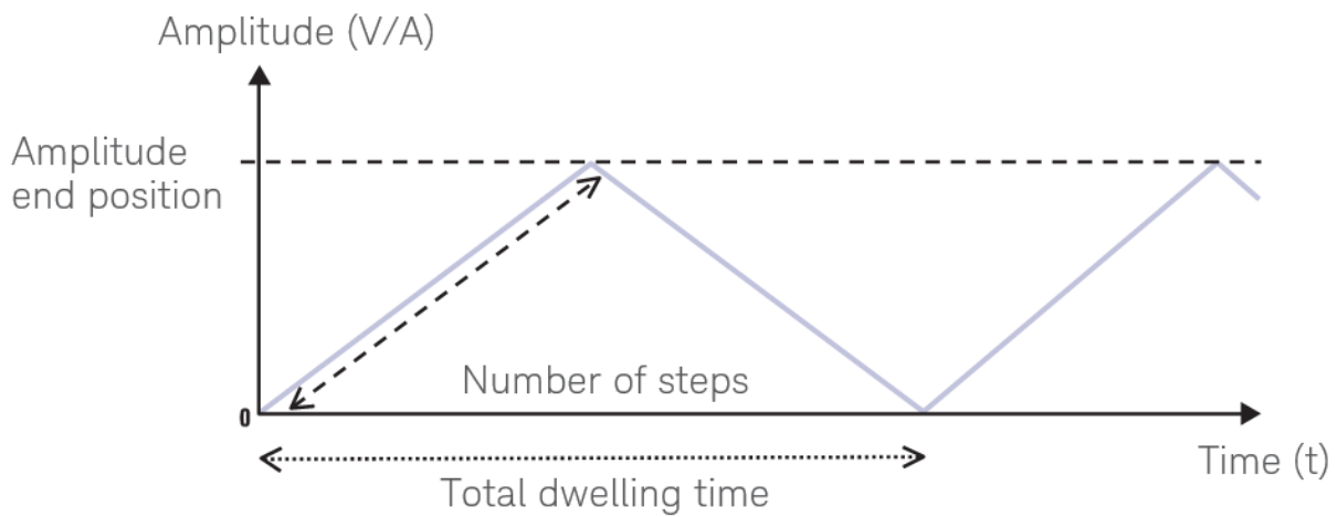
Figure 2. Ramp signal
