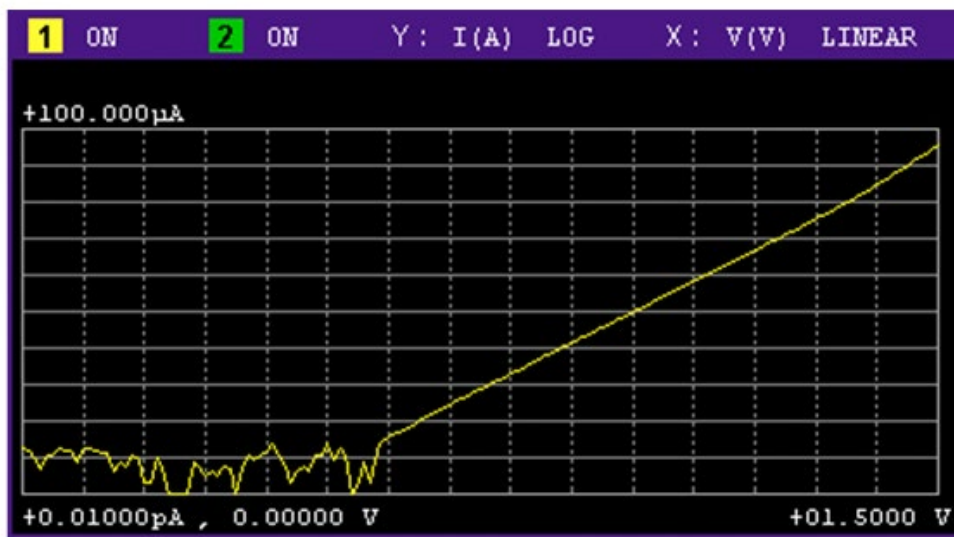
Figure 1. You can make and display accurate low-current measurements directly on the B2900B/BL front panel.
