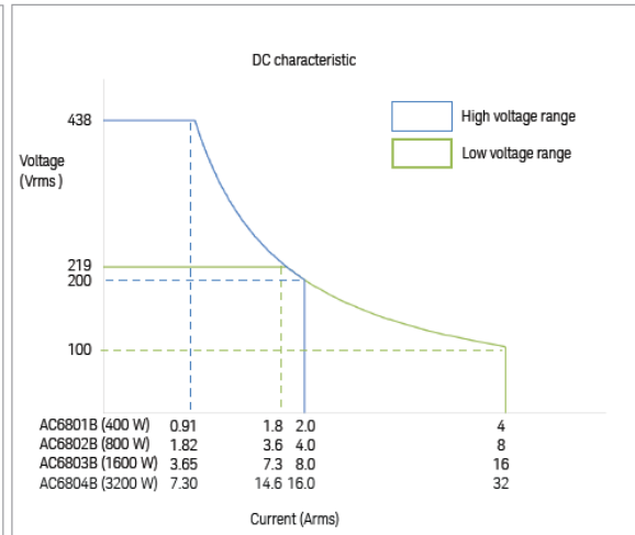
Figure 7. AC6800B steady-state DC output characteristic.
