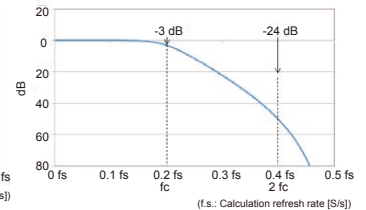
Example IIR-LPF (4th order) frequency characteristics
