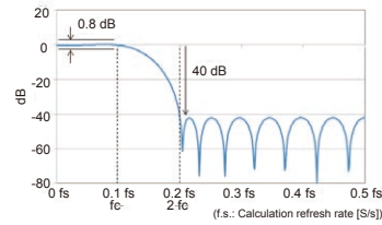
Example FIR-LPF frequency characteristics
